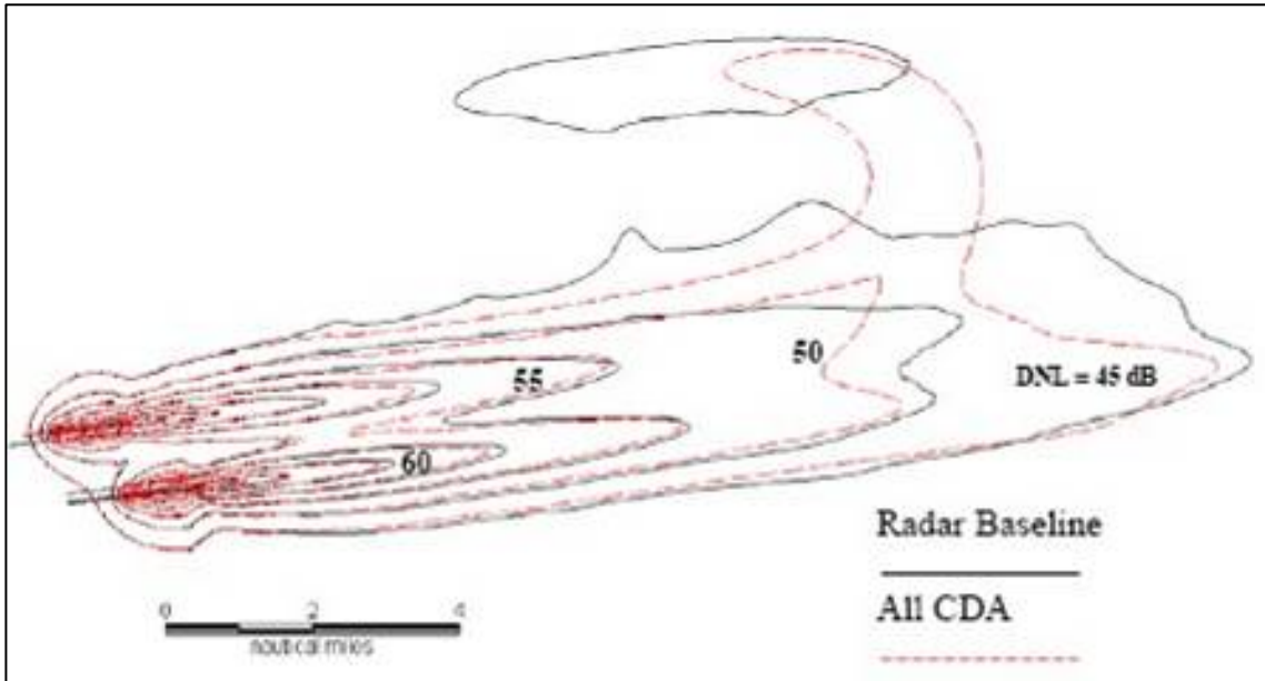
Figure 6: Baseline and All-CDA DNL Contour Overlays
