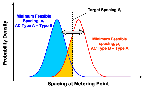
Figure 5: The conditional probability method
