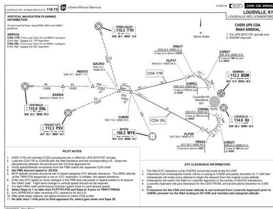
Figure 1: Chart of the KSDF 2004 RNAV CDA
