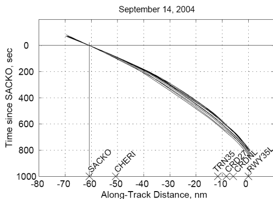
Figure 11: September 14 CDA trajectories
