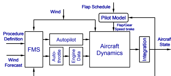
Figure 3: Aircraft simulator block diagram
