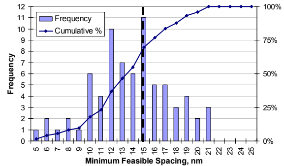
Figure 12: Sample distribution of minimum feasible spacings for the CDA to 35L
