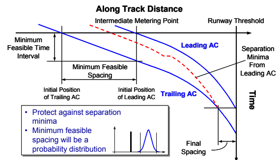
Figure 4: Minimum feasible spacing
