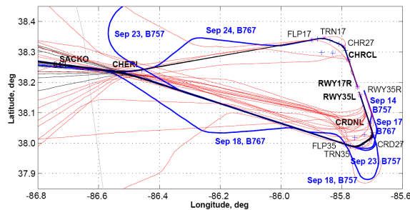
Figure 9: KSDF CDA flight test ground tracks
