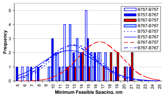
Figure 13: Sample frequency distributions of minimum feasible spacings for different aircraft sequences, CDA to runway 35L
