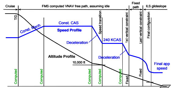
Figure 2: Vertical profile of RNAV CDA
