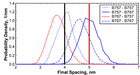
Figure 8: Final spacings given 15 nm at SACKO
