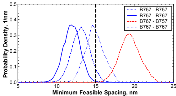
Figure 7: Minimum feasible spacings at SACKO
