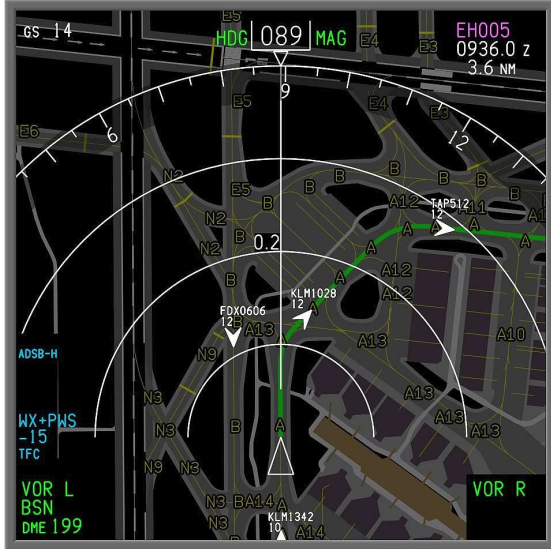
(a) Autonomy level 1 with the AMM, taxi route and CDTI.
