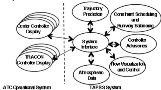
Figure 1. TAPSS simplified functional diagram.
